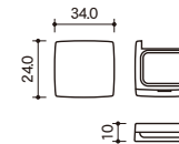
RGI-11 W34.0×D32.0×H10.0
